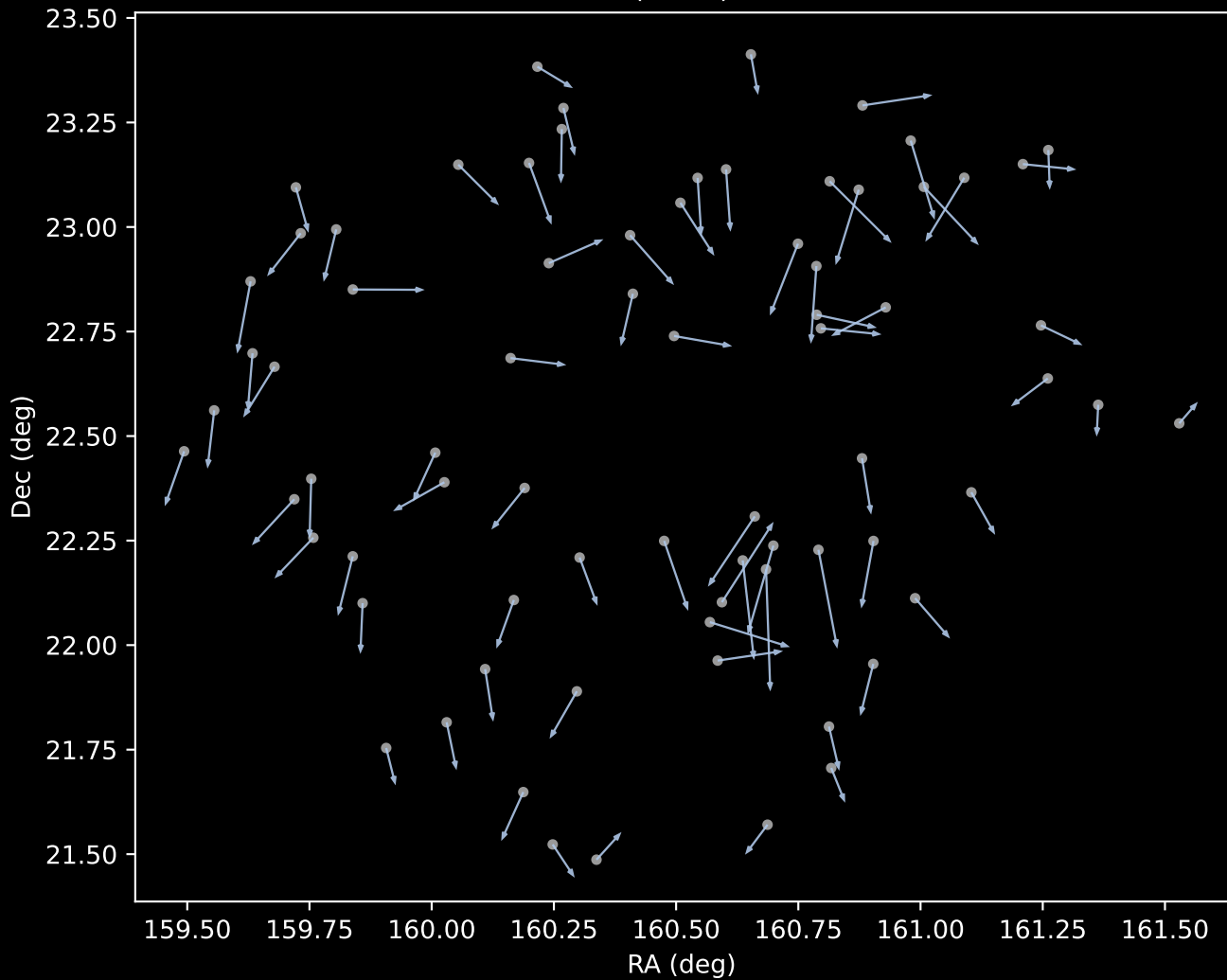
GALAH DR4 Cluster 1 Proper Motion Vectors (n=74)
