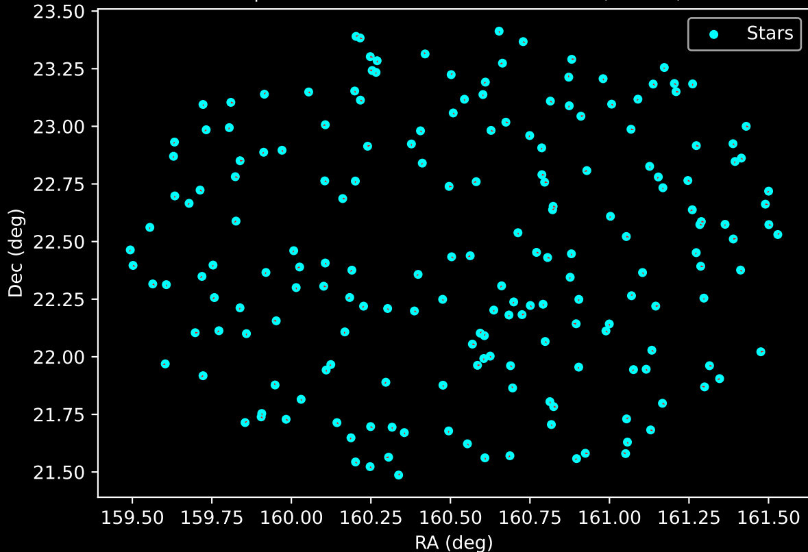
GALAH DR4 Field: [6588] Proper Motion Vectors for Gaia Star Field (n= 190)
