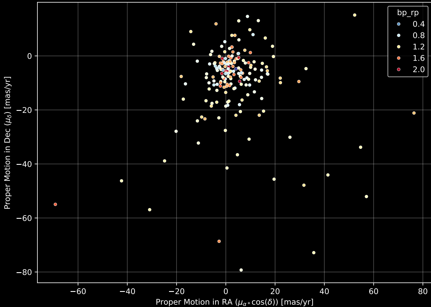
GALAH DR4 Field: [6588] Proper Motion Diagram (n= 190)
