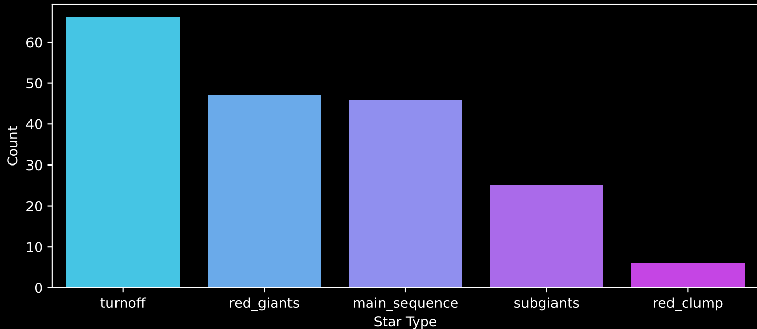
GALAH DR4 Field: [6588] Count plot of Star Type
