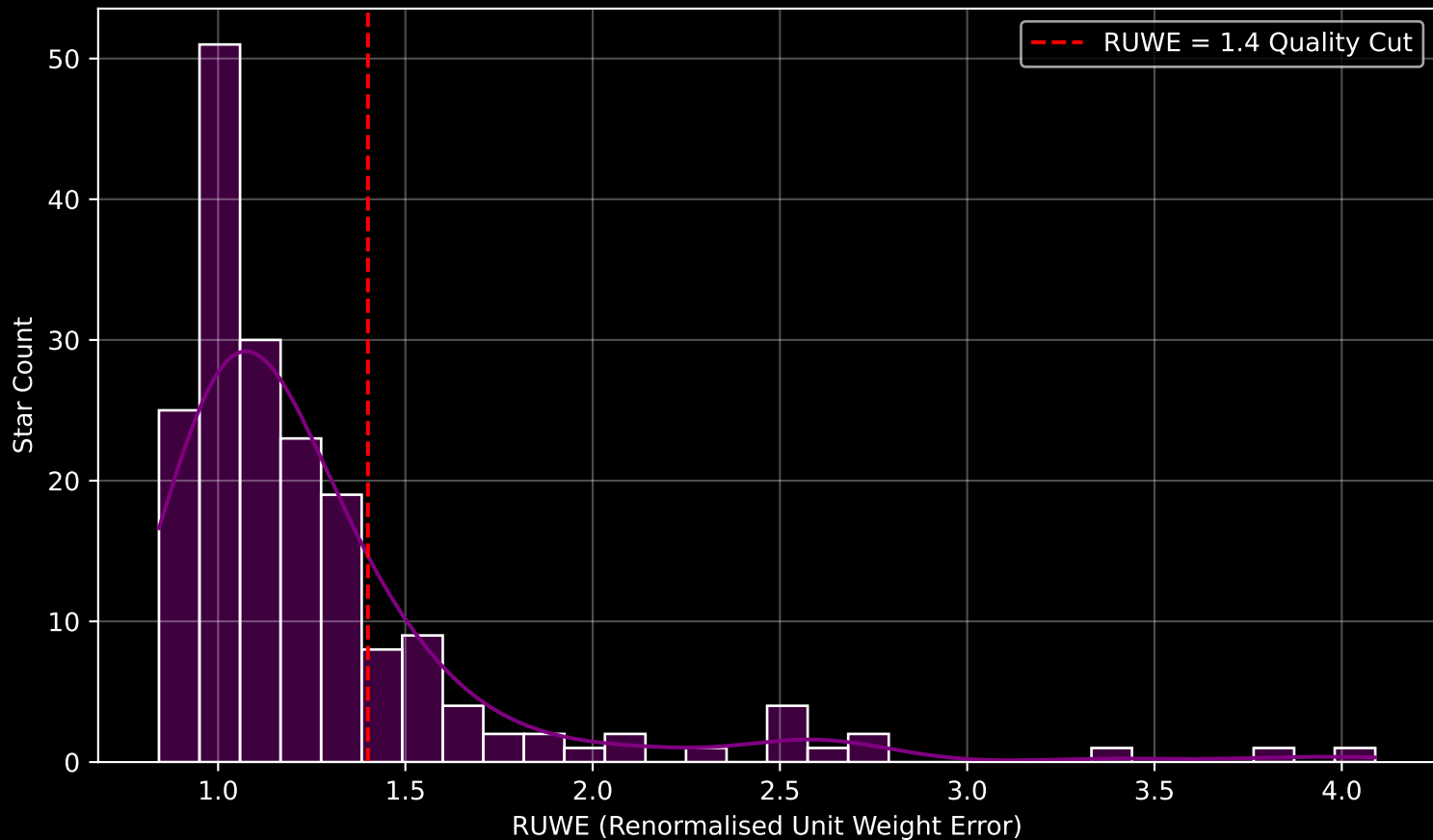
GALAH DR4 Field [6588] RUWE Distribution (n= 187)
